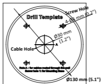
Figure 2-10 Drill Template
