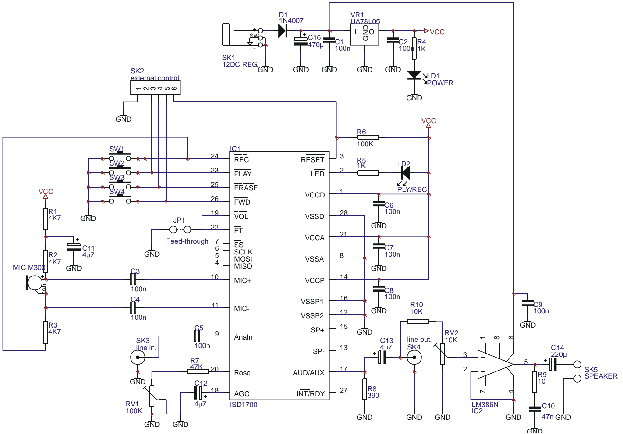
MK195 DIAGRAM
