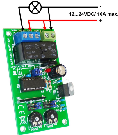
CONNECTION EXAMPLE: LOW VOLTAGE
