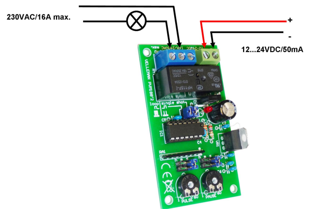
CONNECTION EXAMPLE: AC POWER
